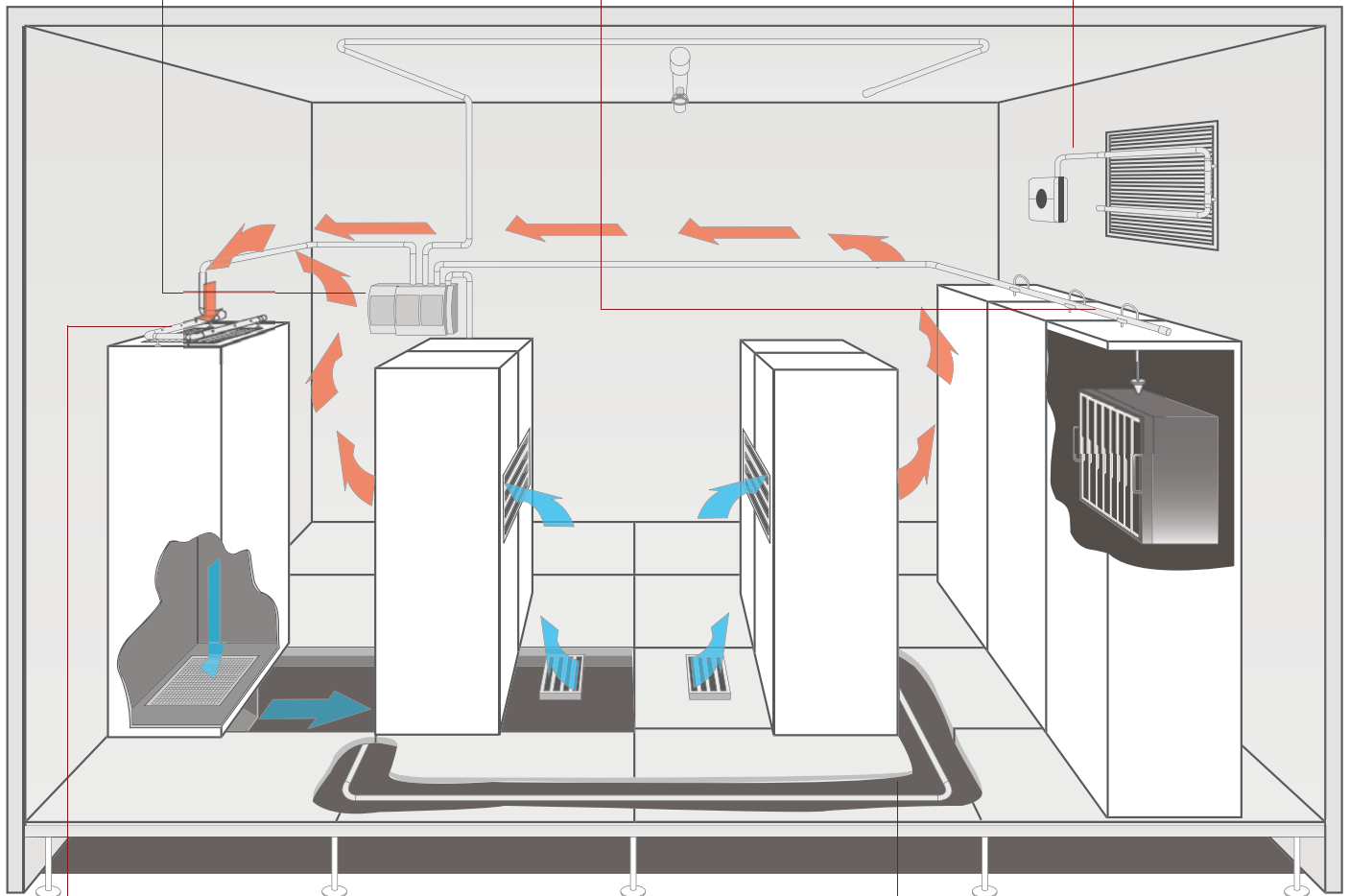
Smoke in an air-conditioned room travels with the airflow to the return air vent, rather than to the ceiling. VESDA sampling pipe can be installed across the vent to detect smoke early.
